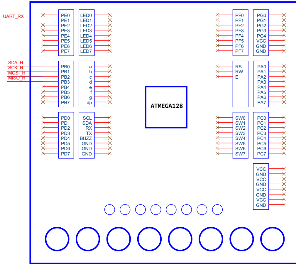
ATMEGA128 Training Board
