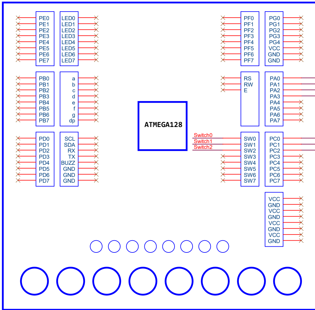
ATmega128 Training Board
