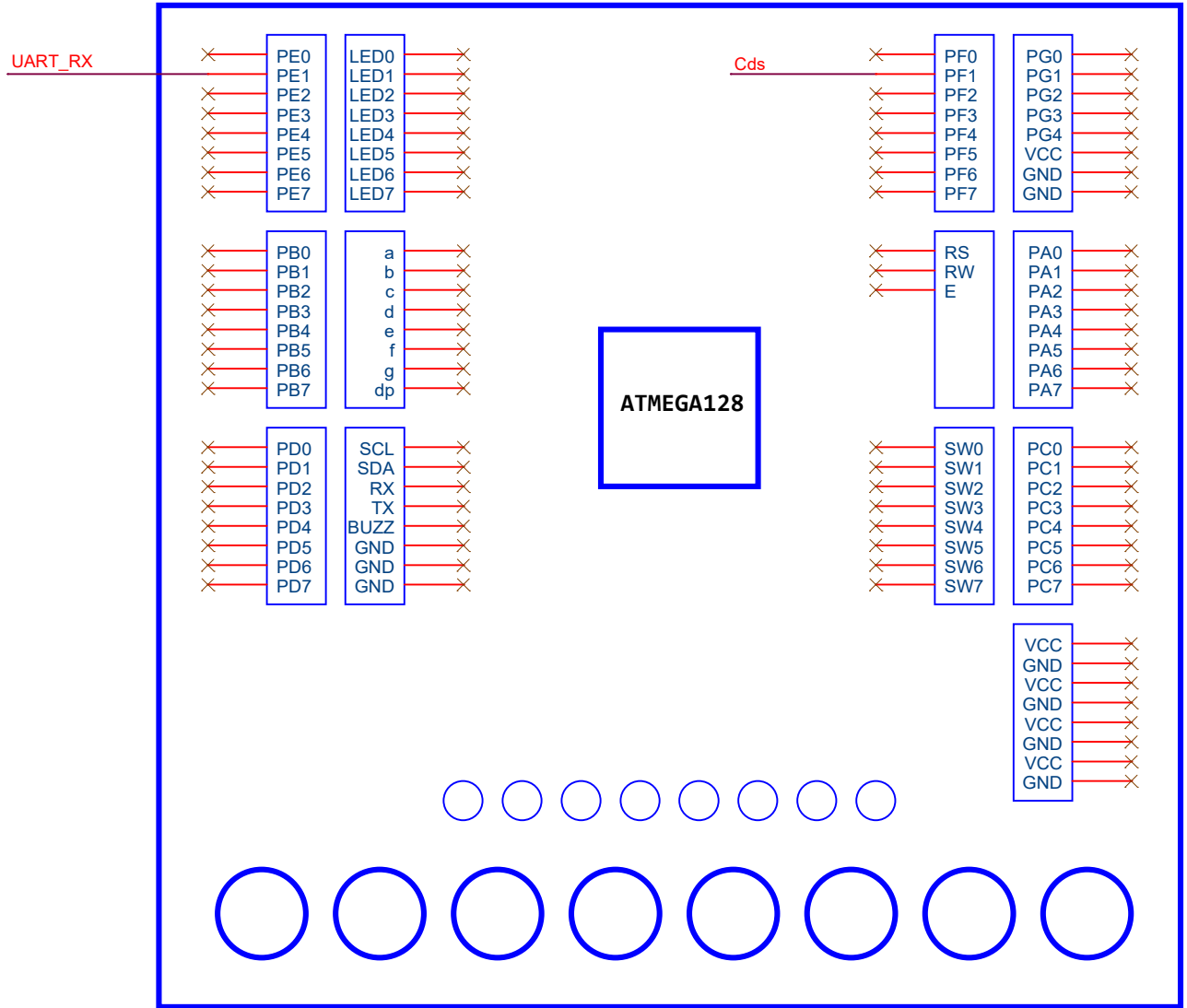
ATMega128 Training Board
