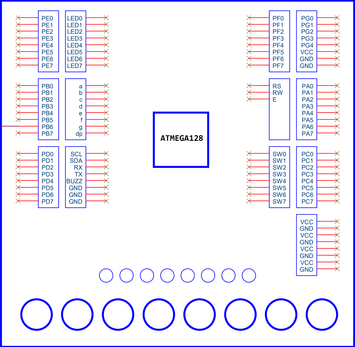
ATMega128 Training Board
