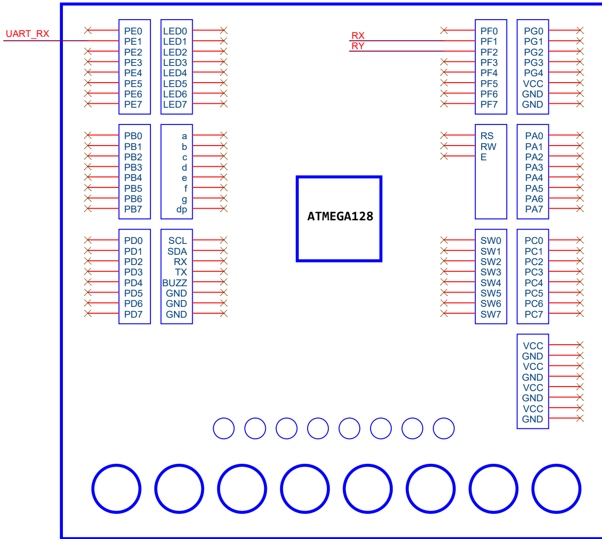
ATMEGA128 Training Board
