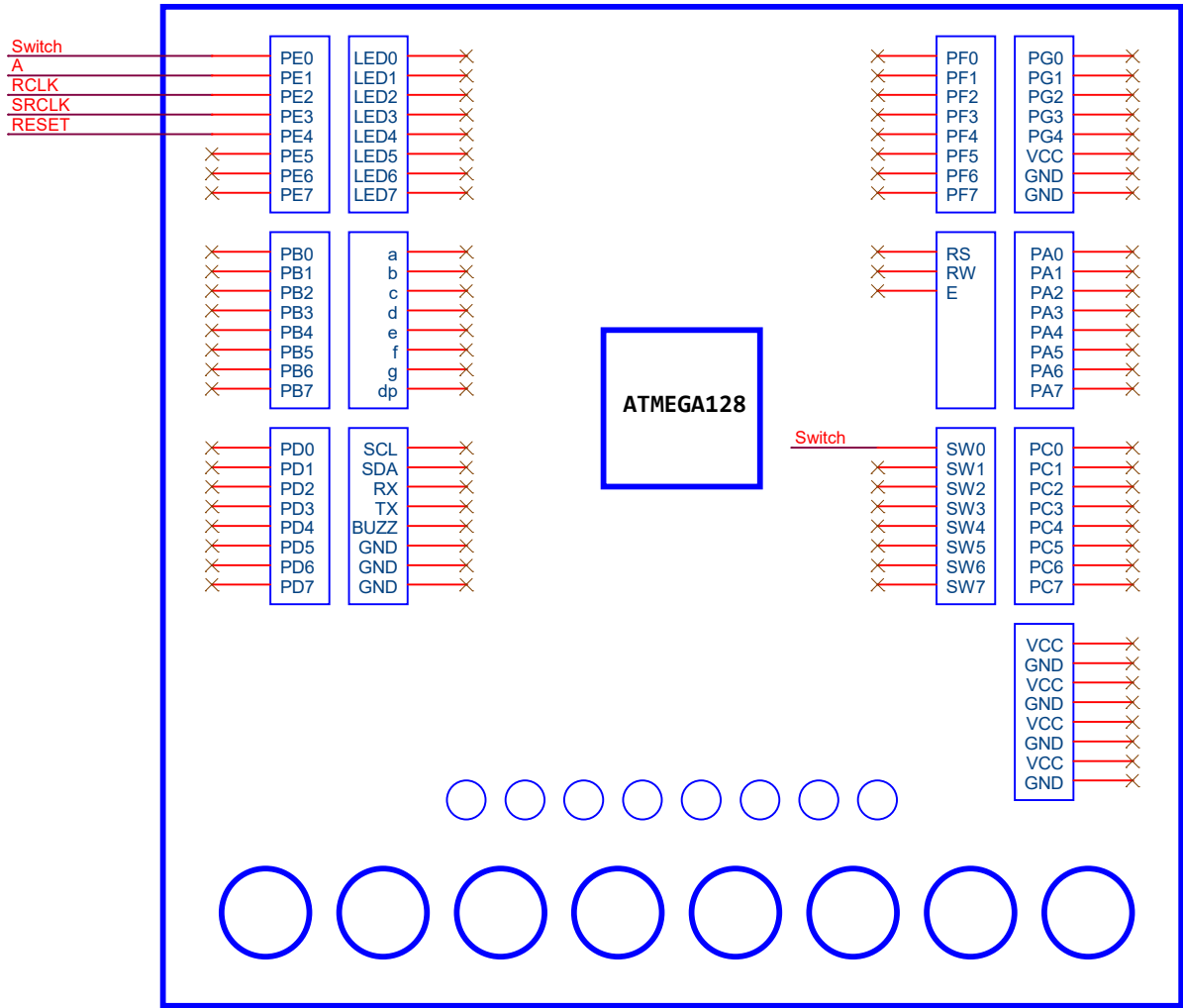
ATMega128 Training Board
