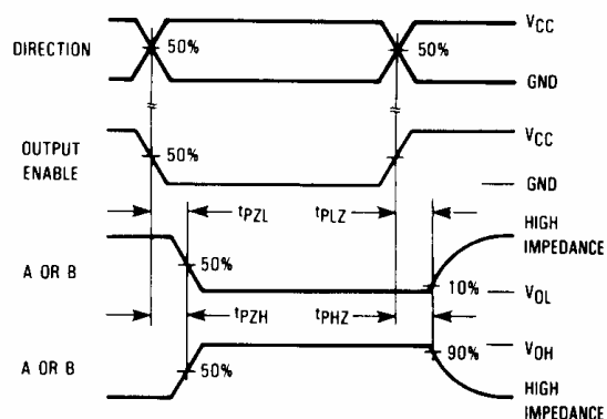
Figure 2. Switching Waveforms
